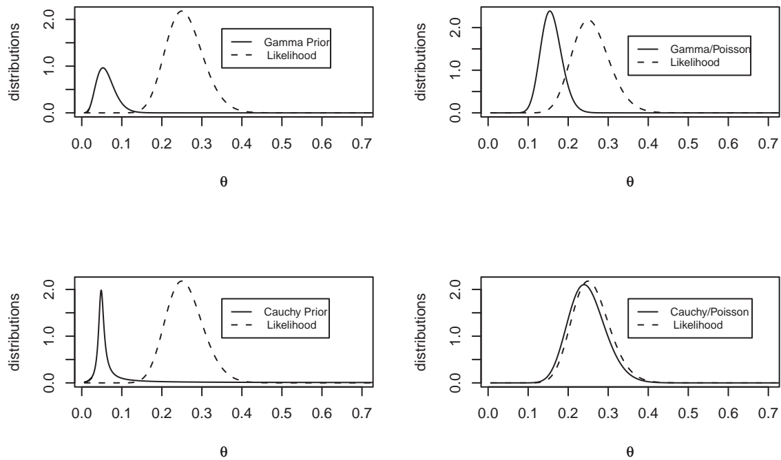
Figure 3 Cauchy/Poisson and Gamma/Poisson when prior and likelihood are in conflict.
