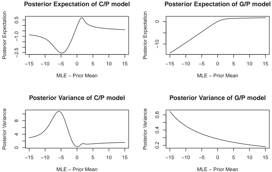
Figure 1 Posterior Expectation and Posterior Variance of the Cauchy/Poisson (C/P) and Gamma/Poisson (G/P) posterior models
