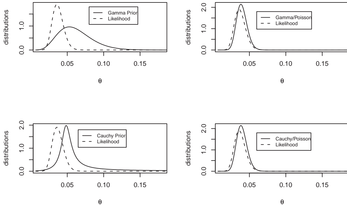
Figure 2 Cauchy/Poisson and Gamma/Poisson when prior and likelihood are consistent.
